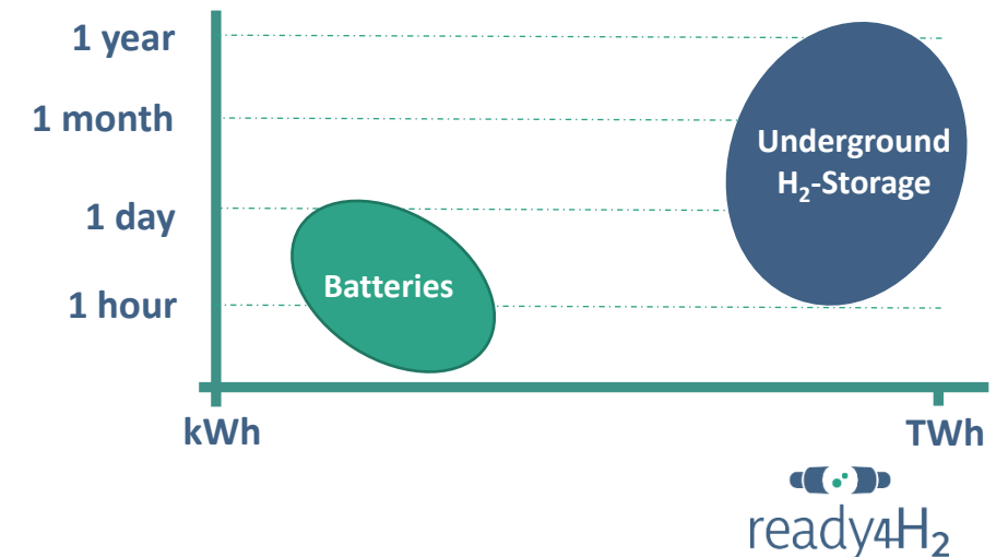
Battery and underground hydrogen storage compared
